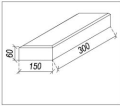
Paving Block ( 150 x 300 x 60 ) used on footpaths and other pedestrian path as specified by design.
