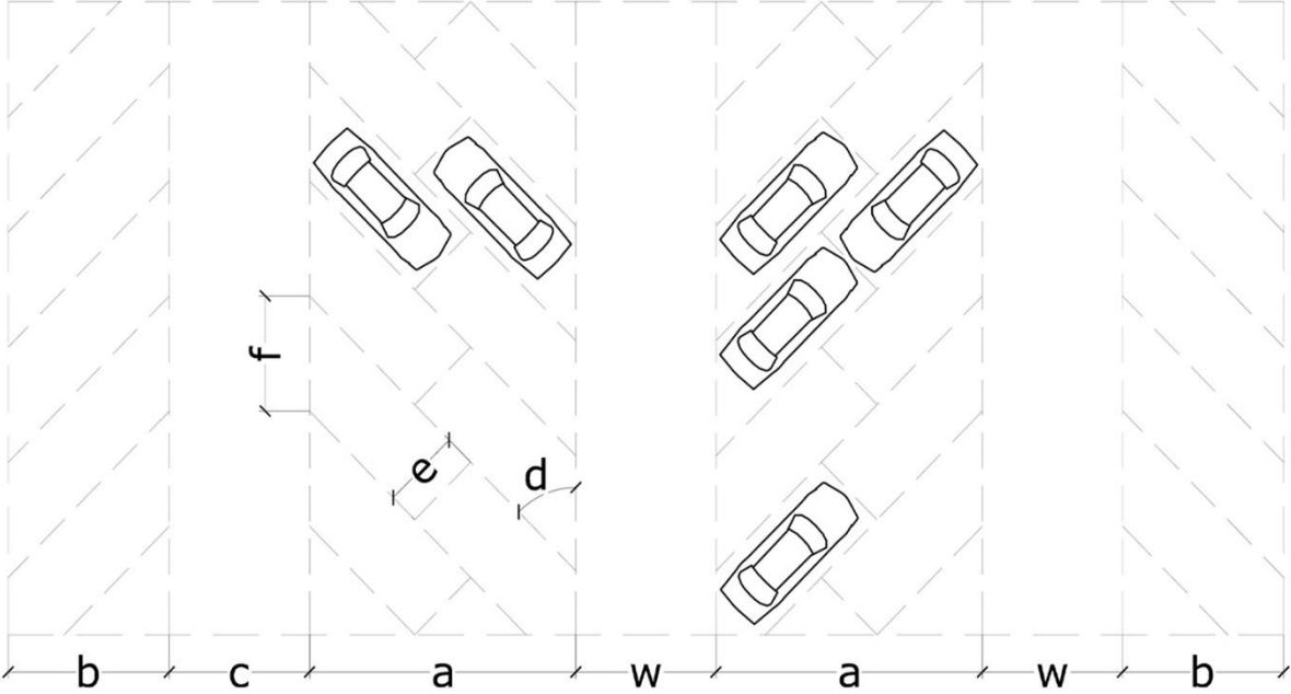
CAR PARKING STANDARDS - long term parking
