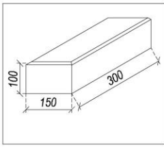
Paving Block ( 150 x 300 x 100 ) used on footpaths where there is also a movement of vehicles.
