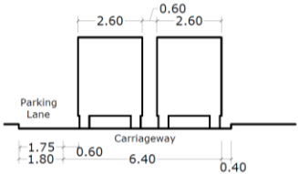
Calculating clearance profile
