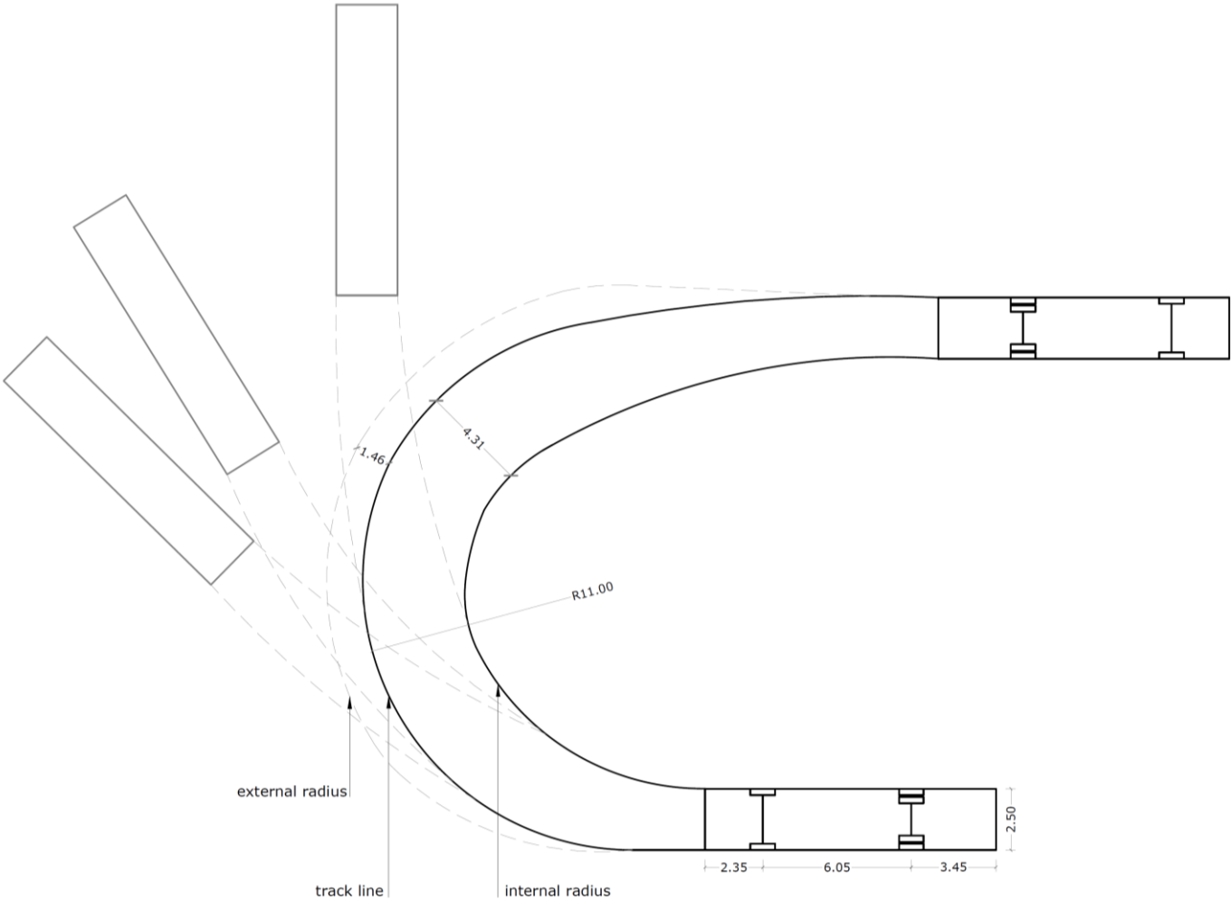
Description of path covered by a bus Speed - 10km/h
