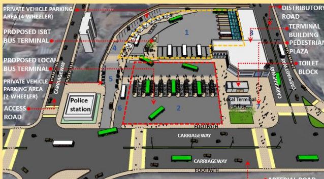
Figure 35: Area allocation for ISBT and Local terminal (Proposal 1)
