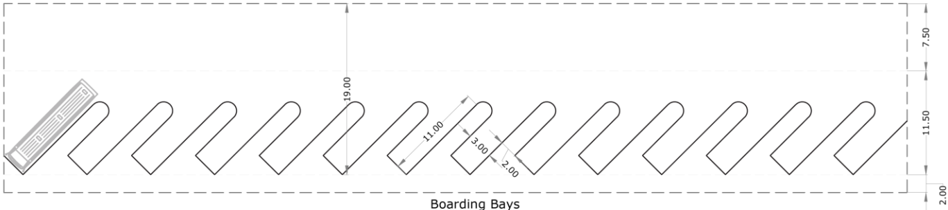
Boarding Bays ANGLED - 45degree
